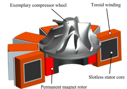
bearingless high-speed motor
