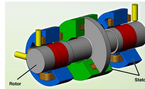
magnetically levitated shaft
