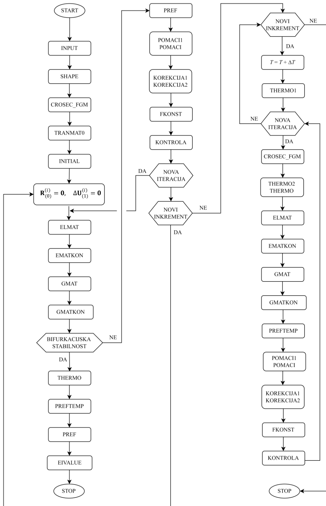
Sl. 5.1 Tijek programa THINWALL FG
